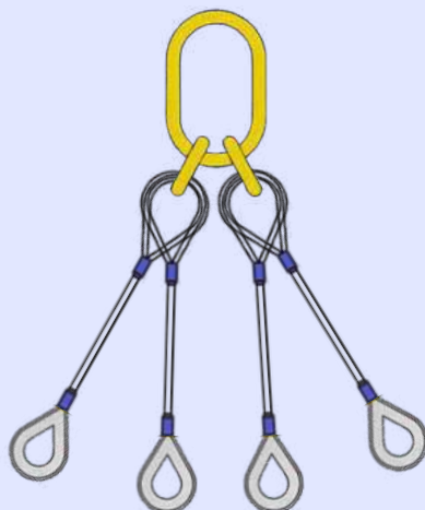
Ref FC-LC4-OS
