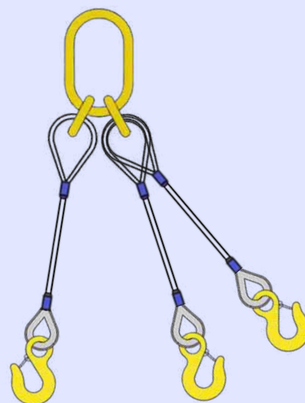
Ref FC-LC3-OSGOT
