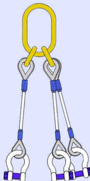
Ref FC-LC3-SSMC
