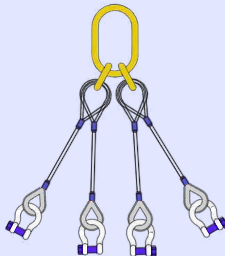
Ref FC-LC4-OSMC
